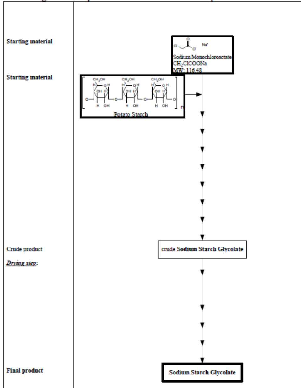
Flow Diagram for Synthesized Sodium Starch Glycolate
