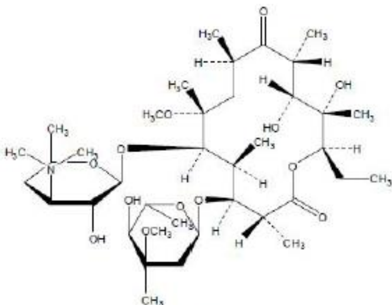
Clarithromycin Chemical Formula: C_{38}H_{59}NO_{13} Molecular Weight: 747.95
