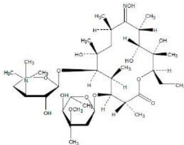
Erythromycin Oxime Chemical Formula: C_{37}H_{68}N_2O_{13} Molecular Weight: 748.04
