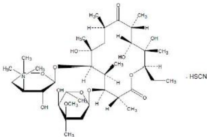
Erythromycin Thiocyanate Chemical Formula: C_{37}H_{67}NO_{13} \cdot HSCN Molecular Weight: 793.02
